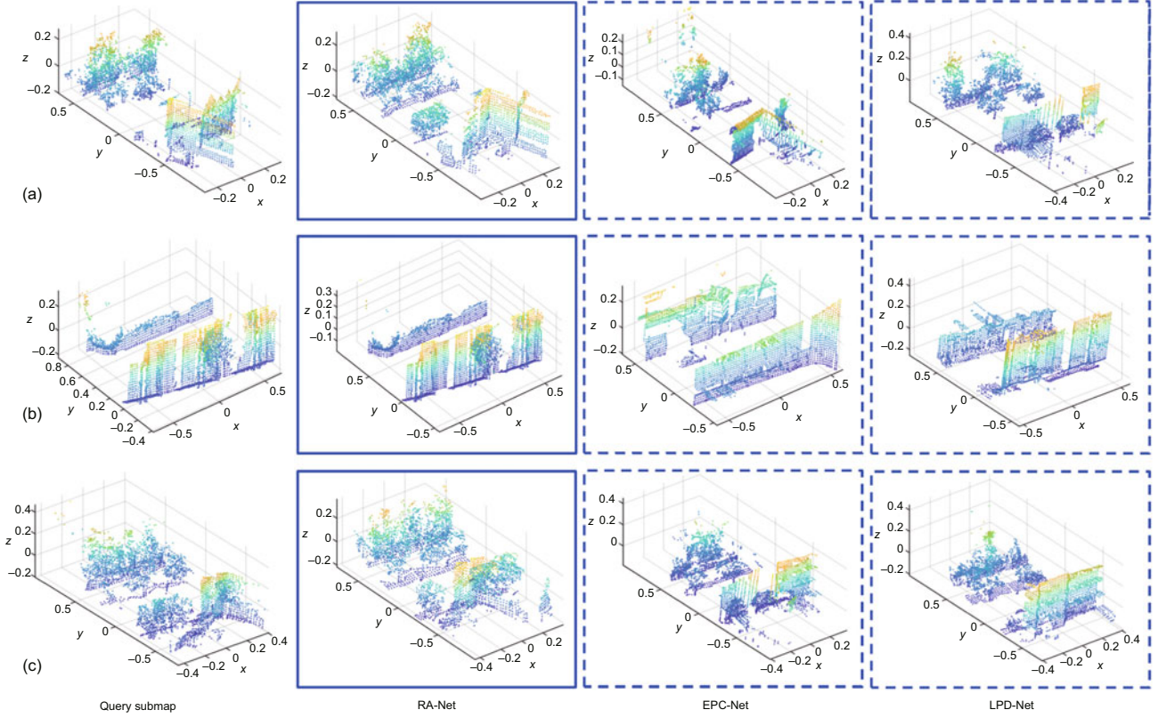
Fig. 7 Comparison of different methods on the Oxford dataset. The first column presents different query submaps, and the subsequent three columns show the retrieval results for our RA-Net, EPC-Net, and LPD-Net. The query point clouds contain structurally diverse trees and incomplete building walls (a), regularly shaped buildings (b), and trees and planes (c). The solid-line quadrilaterals represent successful retrievals, while dotted-line quadrilaterals indicate failures
