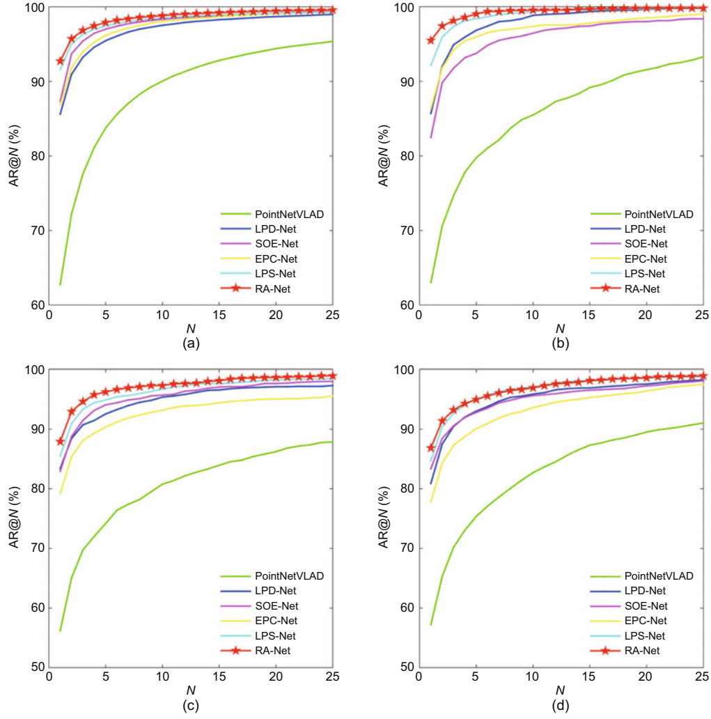
Fig. 4 AR@N of PointNetVLAD, LPD-Net, SOE-Net, EPC-Net, LPS-Net, and RA-Net on the Oxford (a), U.S. (b), R.A. (c), and B.D. (d) datasets
