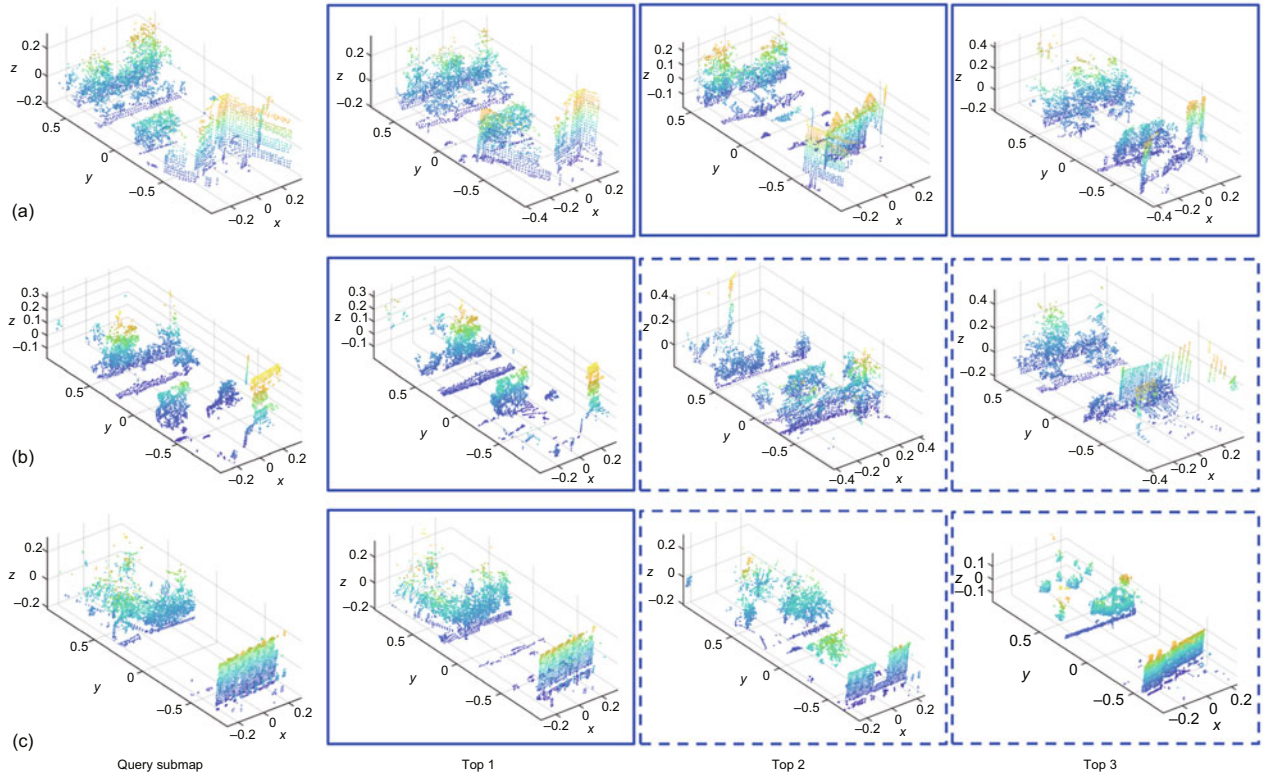
Fig. 5 Visualizations of retrieval results of RA-Net on the Oxford dataset. In these visualizations, the first column displays three different query point clouds, while the following three columns show the top-3 retrieved submaps. The query point clouds contain buildings and trees (a), highly incomplete buildings (b), and low shrubs, a regularly shaped building wall, and curbs (c). The solid-line quadrilaterals denote positive matches, and the dotted-line quadrilaterals denote incorrect matches
