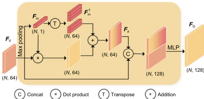
Fig. 3 Network of the GFE module
