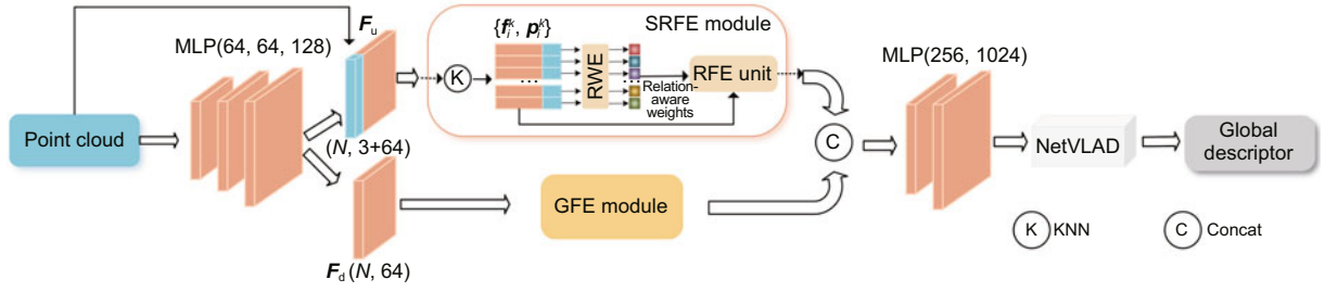
Fig. 1 Overview of the RA-Net architecture. N denotes the number of points, and k denotes the number of nearest neighbors. KNN: k -nearest neighbor
