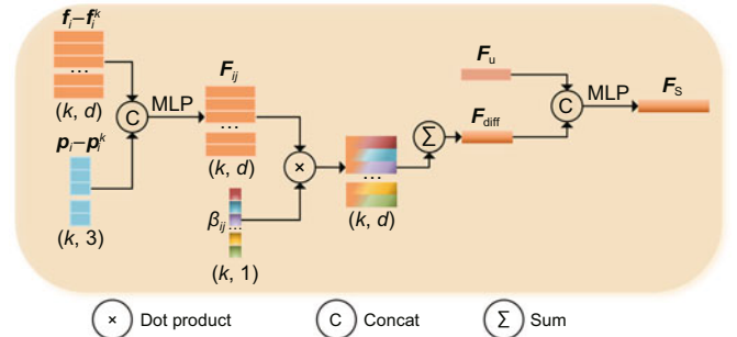
Fig. 2 Network of the RFE unit. d denotes the dimension of the features
